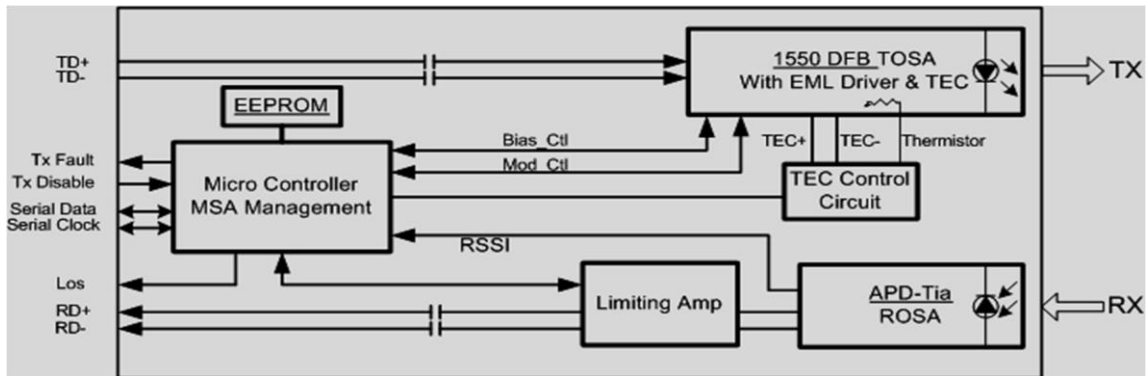
Figure 5: Module Block Diagram
