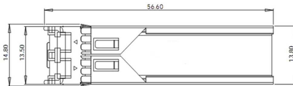
Mechanical Drawing
