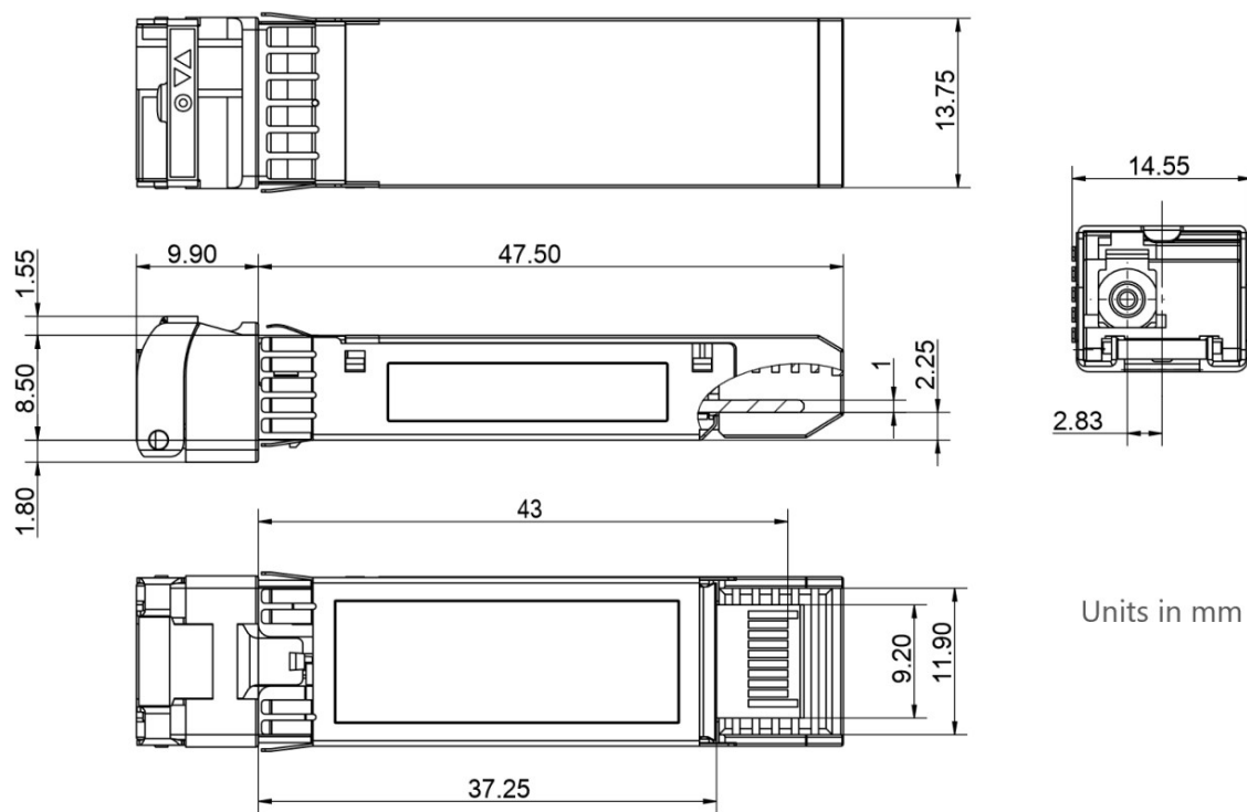
Figure2. Mechanical Outline
