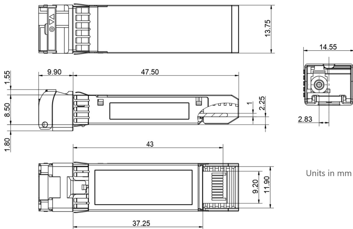
Figure2. Mechanical Outline
