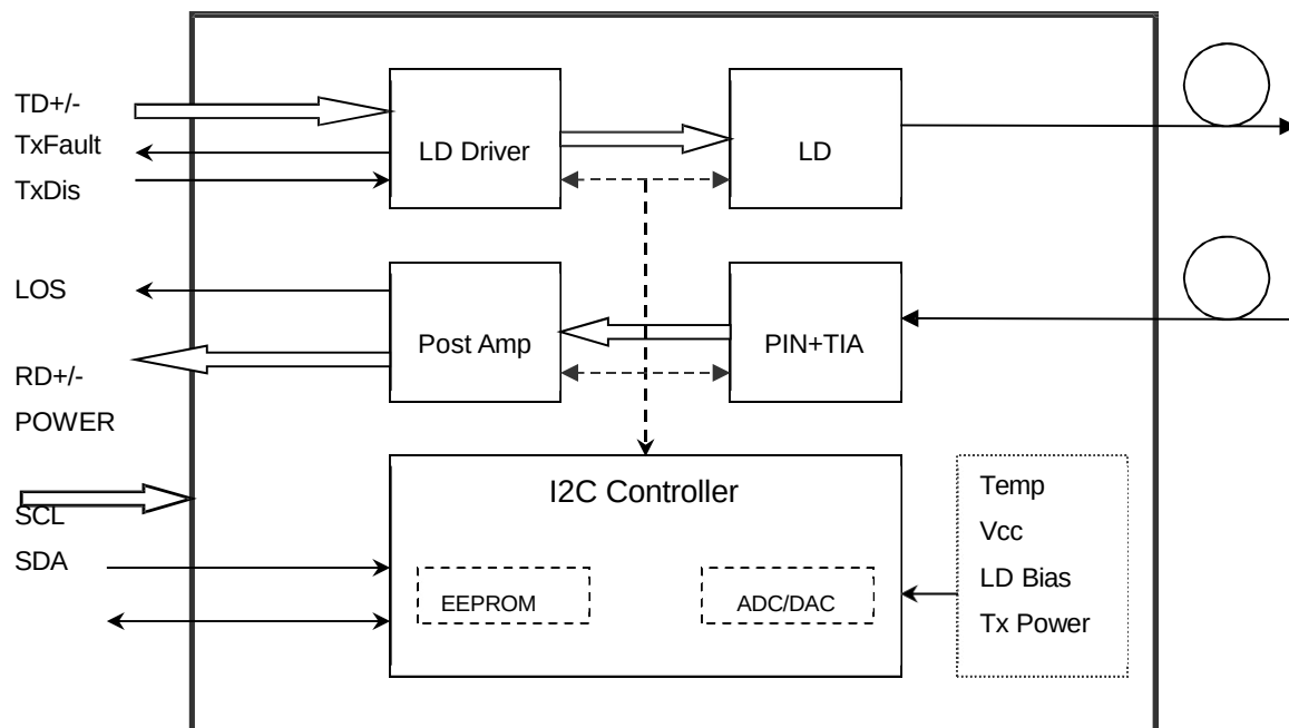
Transceiver functional diagram
