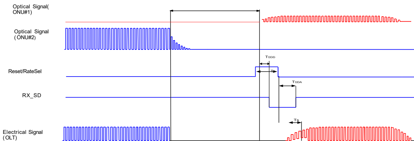
Figure 3 Timing Parameter Definitions in XGS-PON Burst Mode Sequence
