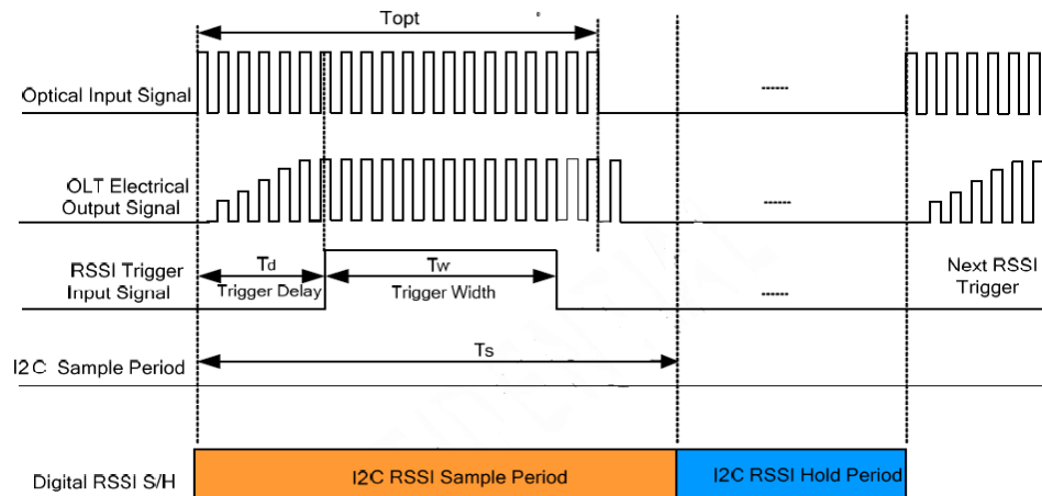
Figure 6 Timing Parameter Definitions in RSSI Trigger
