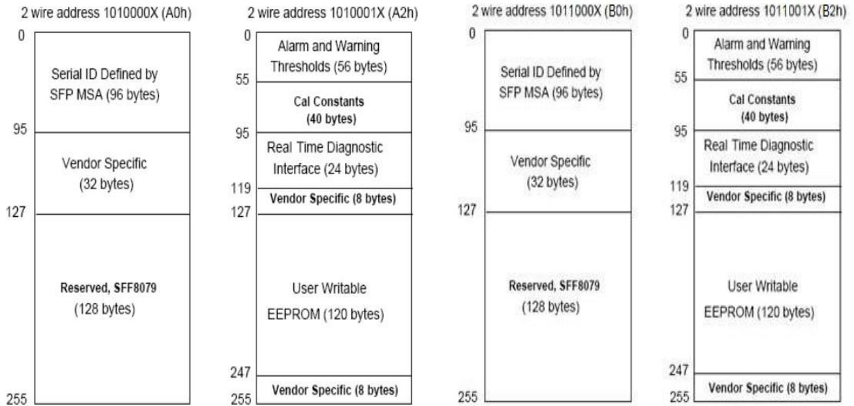
Figure 10 EEPROM Memory Map Specific Data Field Descriptions
