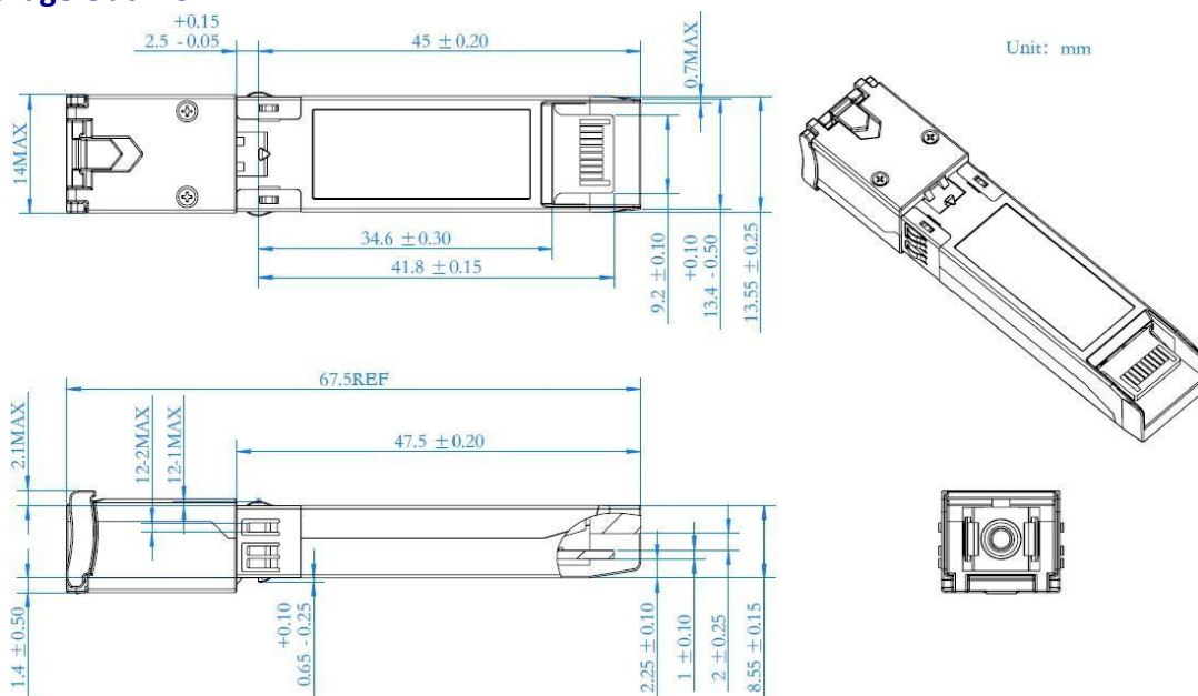
Figure 8 Package Outline
